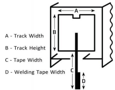
8SY Track Profile
