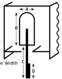
8SY Track Profile
