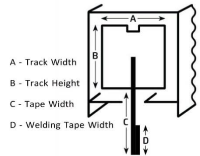
3SY Track Profile
