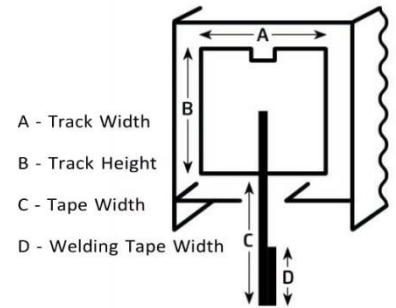
10SY Track Profile
